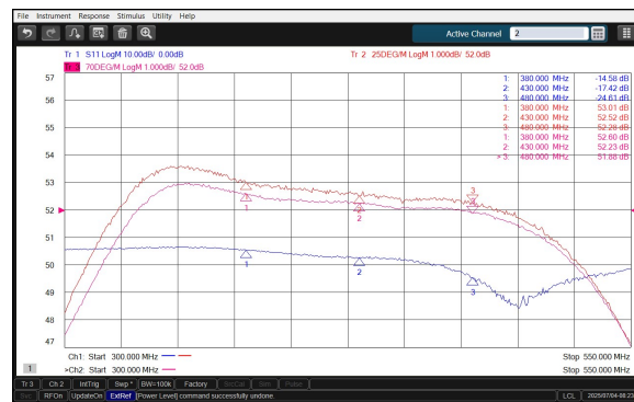
Gain compression at 20W output
