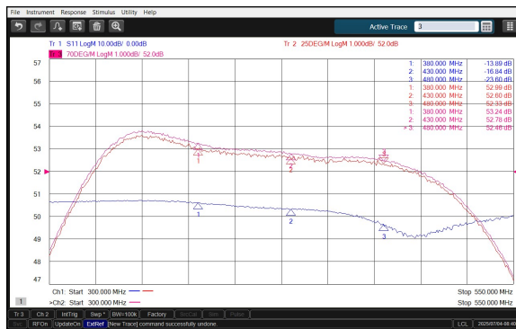
Gain / IRL vs frequency (25°C & 70°C)
