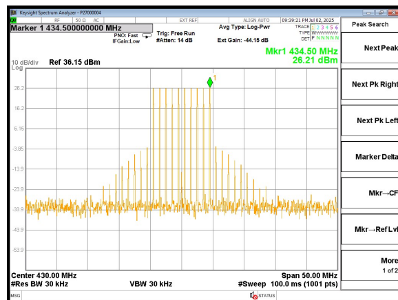
10 tones, 40 W peak, f=430 MHz, peaked phases
