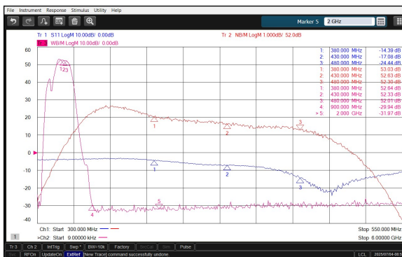
Wideband response
